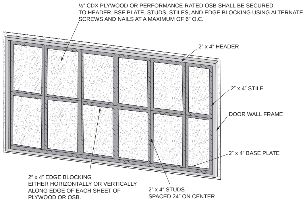
FIGURE A103.1(2)—BOARDING OF DOOR WALL
